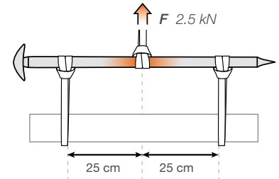
Pull Test
