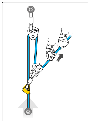
Pulley System
