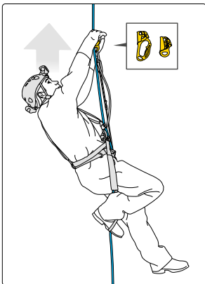
Rope ascent with hand ascender installed above the user
