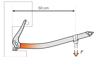
Shaft Insertion Strength Test
