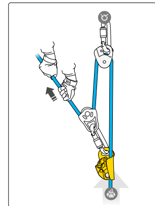
Pulley system with a BASIC ascender
